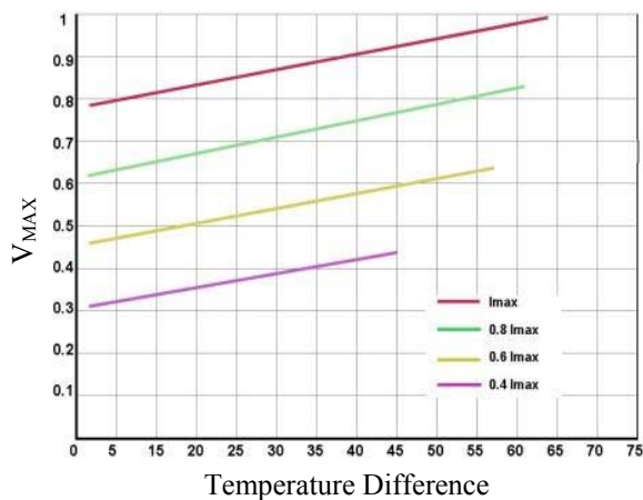
Figure 4. V_{MAX} vs. Temperature Difference
