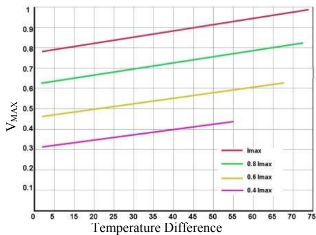
Figure 8. V_{MAX} vs. Temperature Difference
