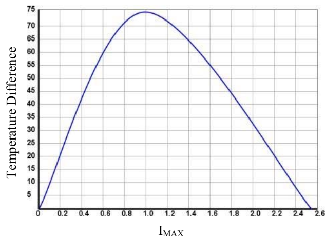
Figure 7. Temperature Difference vs. I_{MAX}
