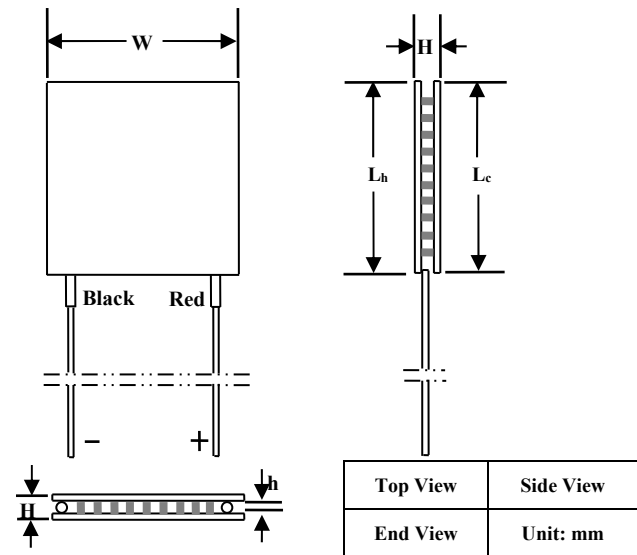
Figure 11. Mechanical Dimensions of Non-sealed ATE1-17
