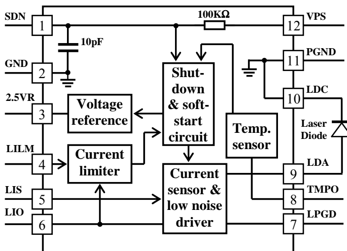
Figure 3 Block Diagram
