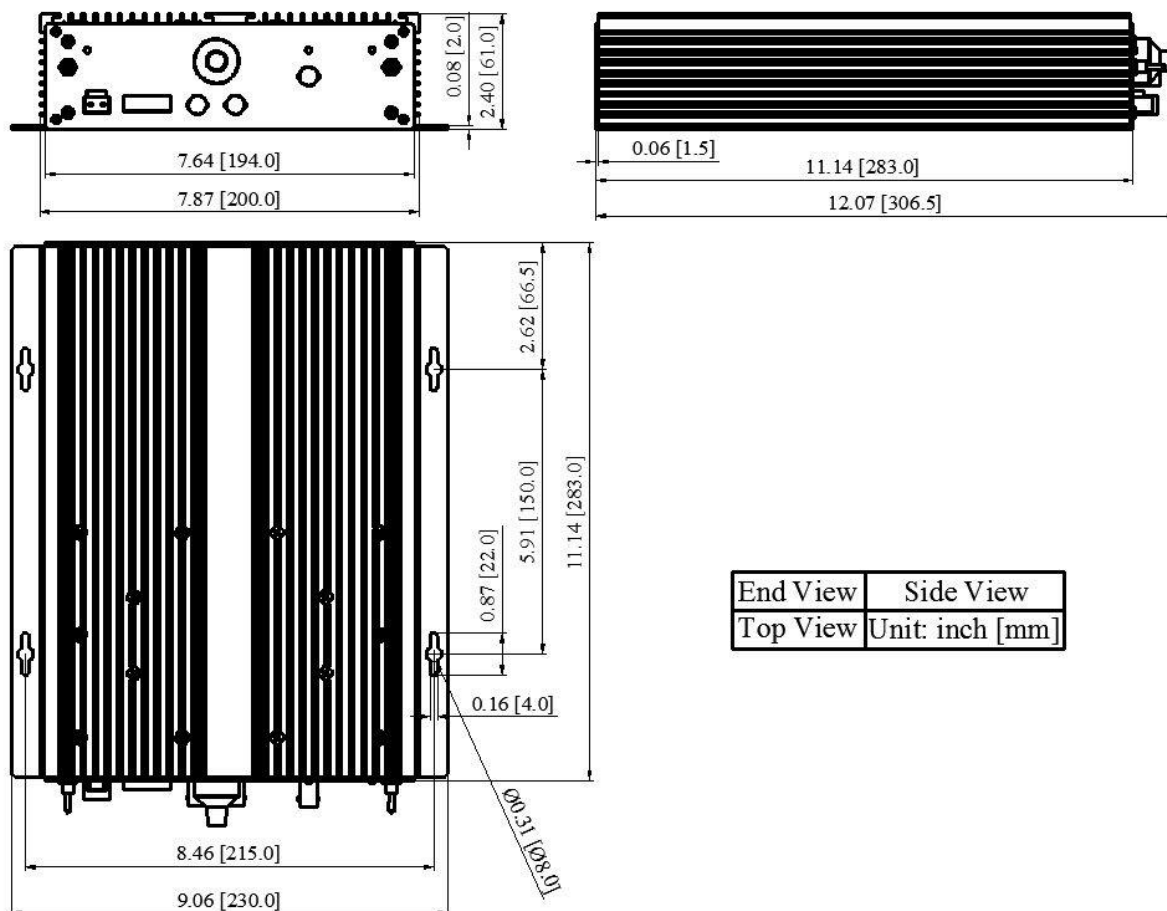
Figure 33. Dimensions of AHVAPN2000V20MA
