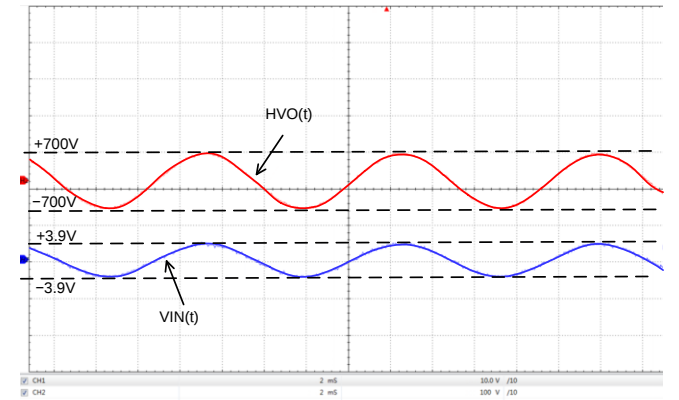
Figure 31. Input vs. Output with Sine Wave
