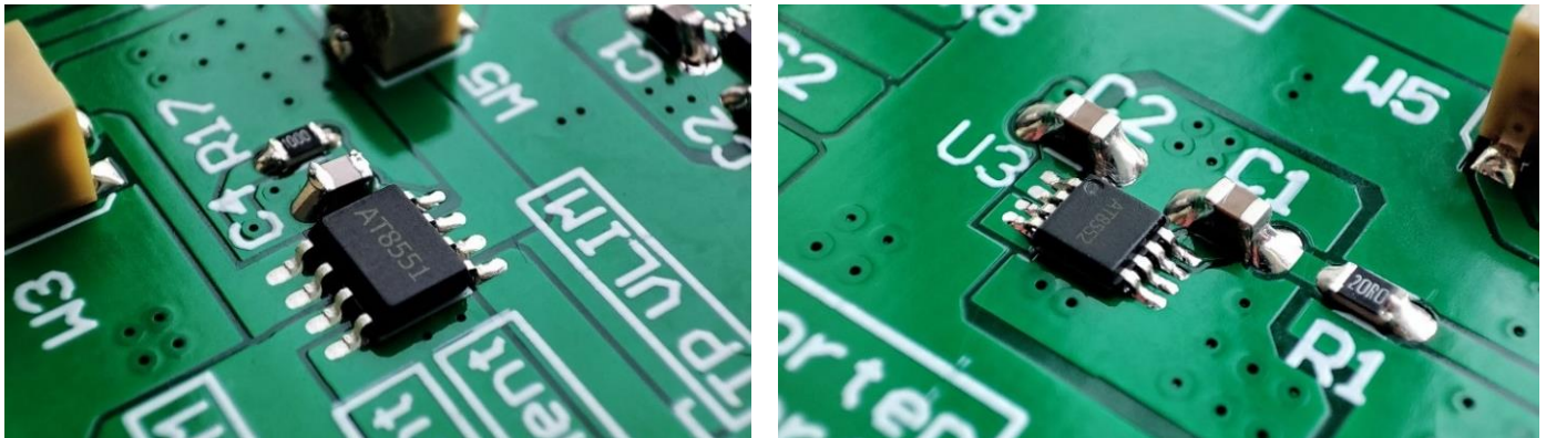
Figure 1. Physical Photos of AT8551
