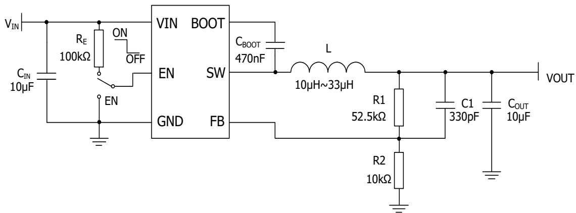
Figure 4. Typical Application Circuit
