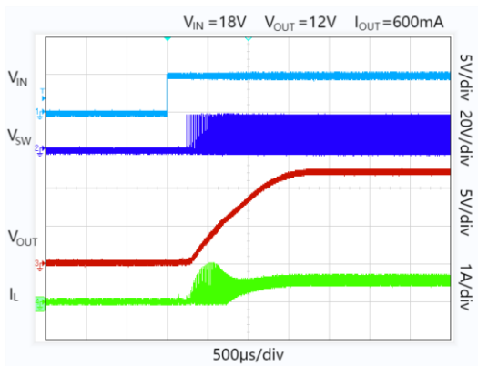
Figure 9. Power-Up
