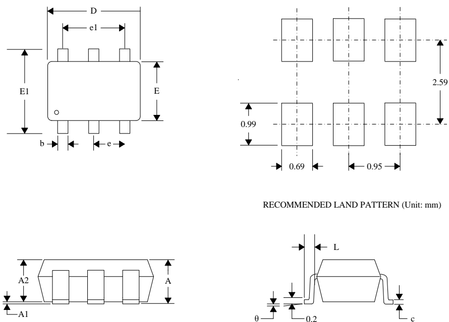
Figure 25. Dimensions
