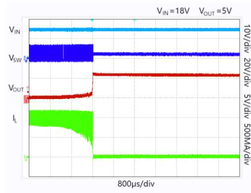
Figure 12. Short-Circuit Recovery
