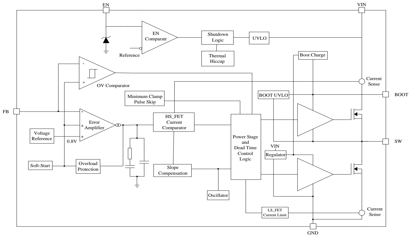
Figure 22. Block Diagram
