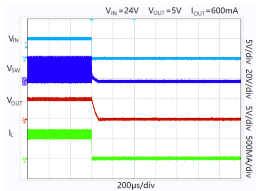
Figure 14. Power-Down
