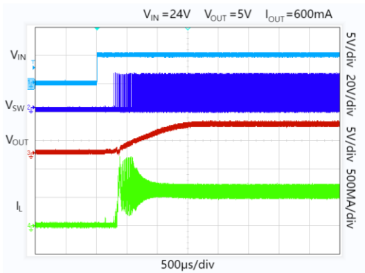
Figure 13. Power-Up
