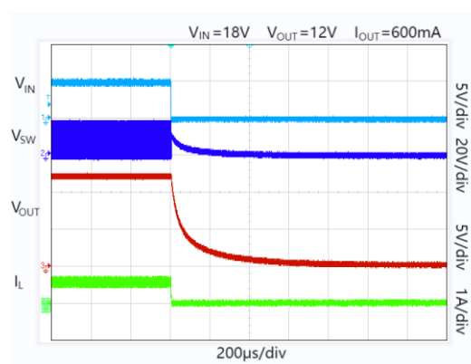
Figure 10. Power-Down
