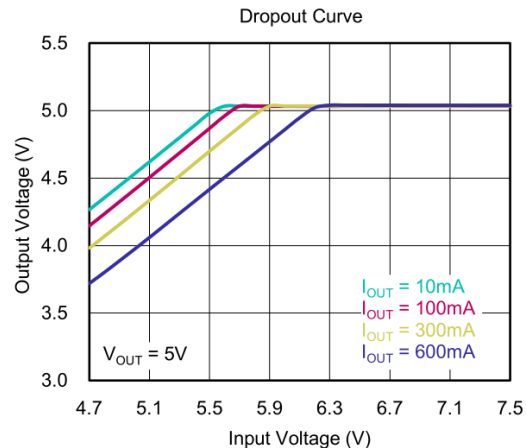
Figure 21. Dropout Curve
