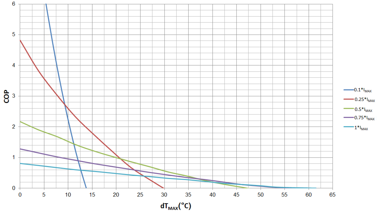
Figure 8. COP vs. dT_{MAX}
