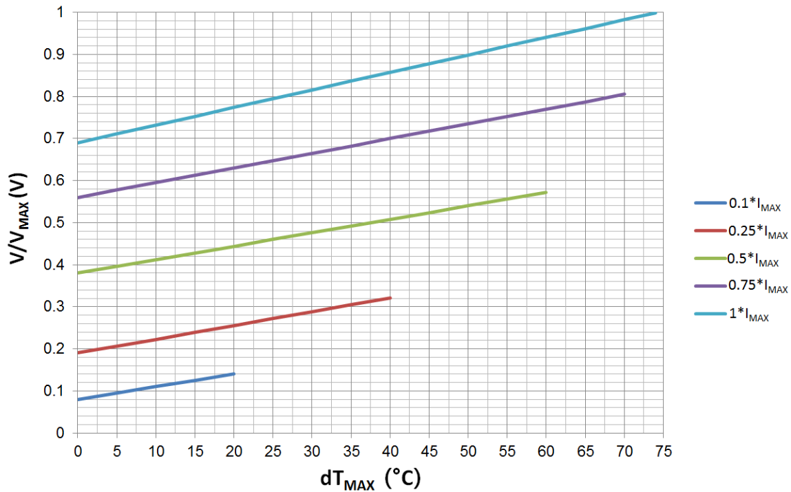
Figure 3. V/V_{MAX} vs. dT_{MAX}
