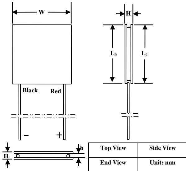
Figure 10. Mechanical Dimensions of Sealed ATE1-07
