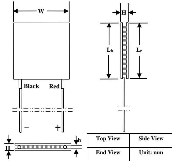
Figure 11. Mechanical Dimensions of Non-sealed ATE1-07
