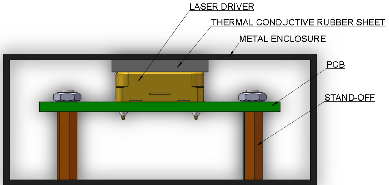
Figure 10.1 Transferring Heat with Metal Enclosure
