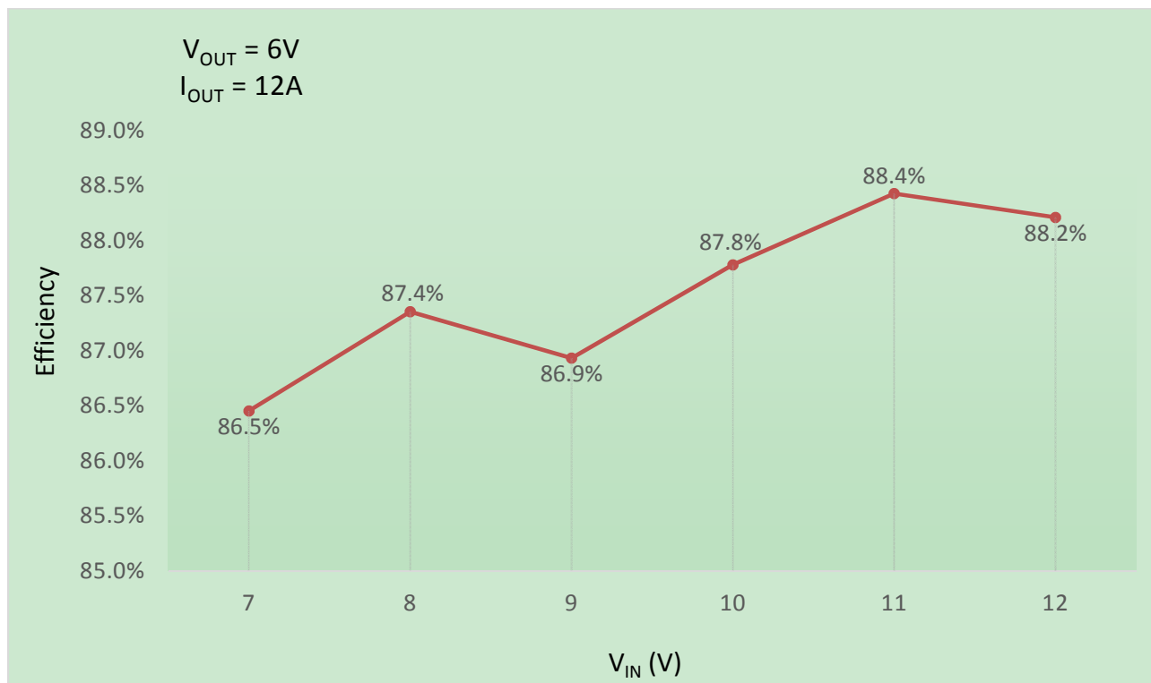
Figure 6. Efficiency vs. V_{OUT} and V_{IN}
