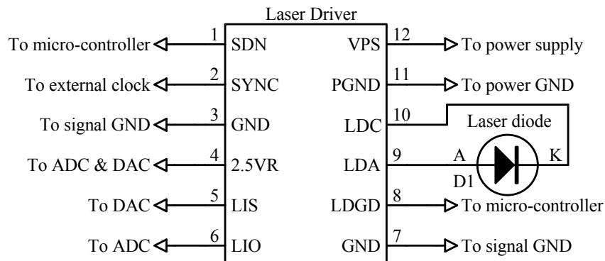
Figure 5. A Typical Micro-processor-based Application Schematic
