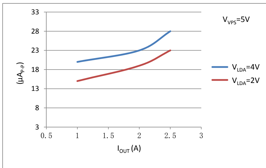
Figure 7. 2. I_{OUT} vs. Output Current Noise@0.1Hz~10Hz
