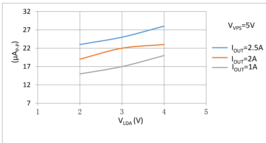
Figure 7. 1. V_{LDA} vs. Output Current Noise@0.1Hz~10Hz
