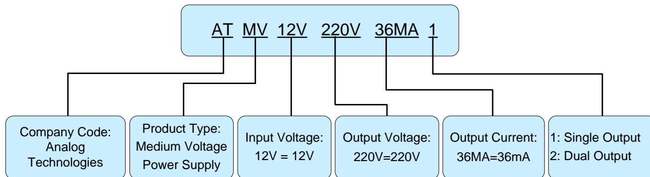
Figure 7. Naming Convention of ATMV12V220V36MA1
