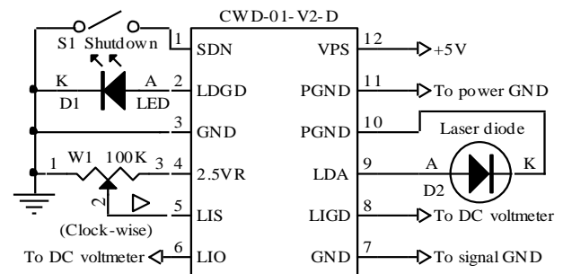
Figure 4. A Typical Stand-alone Application Schematic
