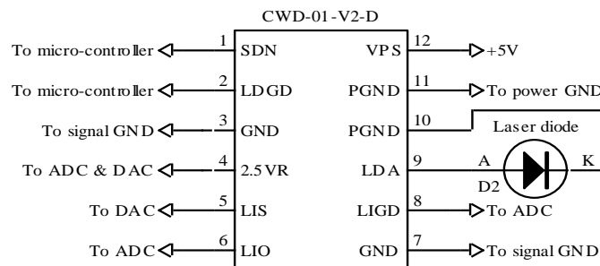
Figure 5. A Typical Micro-processor-based Application Monitoring the Output Current
