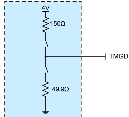
Figure 19. Output Equivalent Circuit for TMGD Pin
