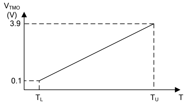
Figure 11. Linear Relationship between V_{\text{TMO}} and Temperature
