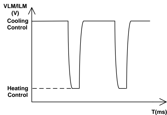
Figure 23. The Waveform on the VLM or ILM Pin @ SB State
