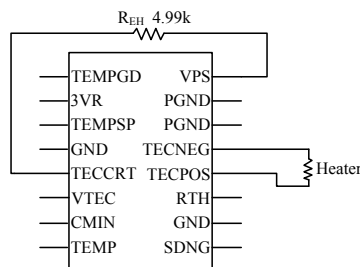
Figure 6.2. Driving a Heater for <3.3V @ ≤3A
