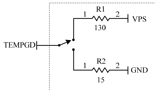
Figure 15. Internal Equivalent Circuit on TEMPGD Pin
