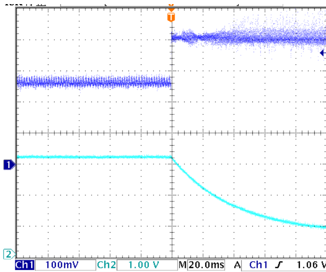
Figure 13. V_{TEC} & V_{TMO} Waveforms
