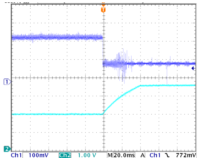
Figure 13. V_{TEC} & V_{TMO} Waveforms
