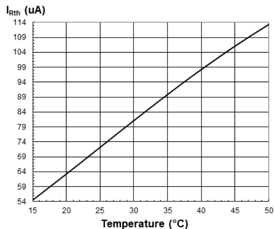
Figure 9. I_{Rth} vs. Temperature
