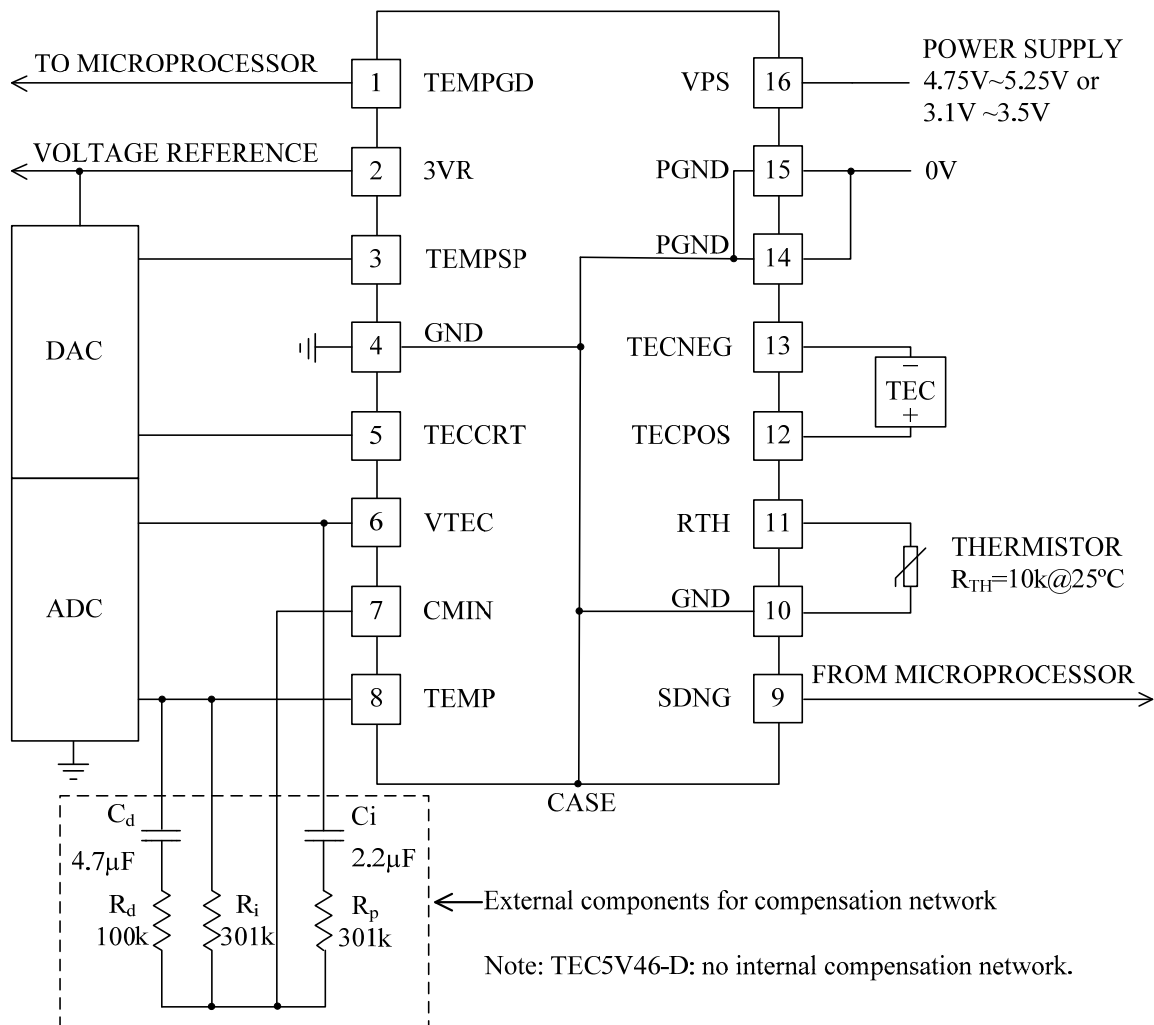
Figure 4. TEC Controller Connections
