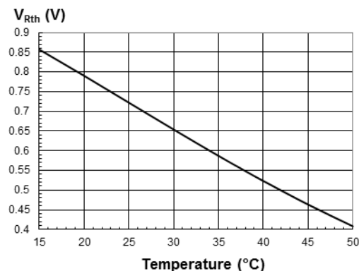
Figure 10. V_{Rth} vs. Temperature
