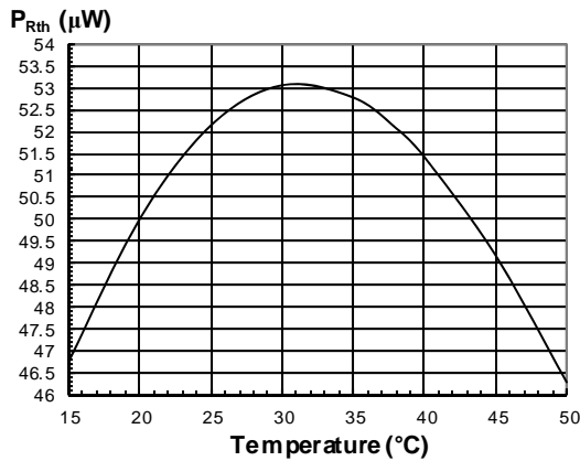
Figure 11. P_{Rth} vs. Temperature
