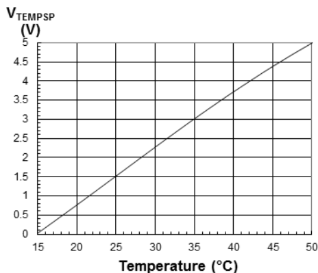
Figure 8. TEMPSP vs. Temperature
