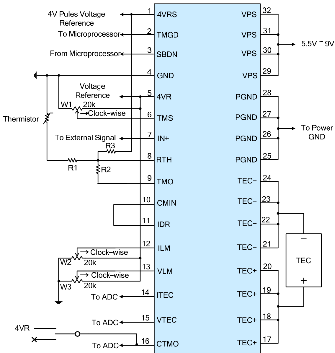
Figure 8.2. Connection for TEC9V15ADAPID & TEC9V15ASAPID
