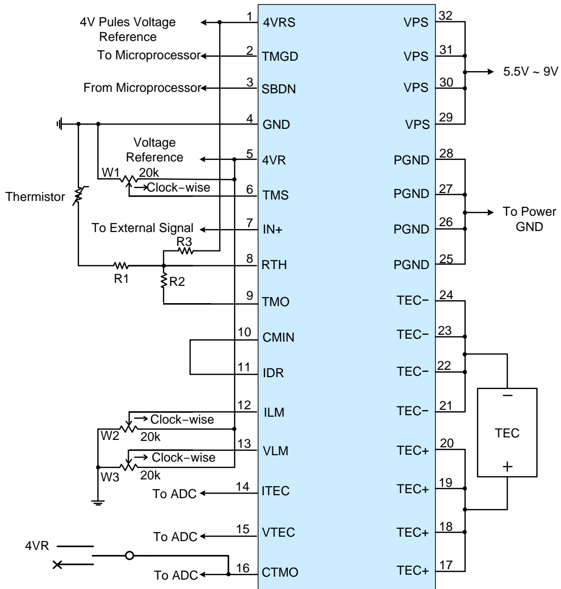
Figure 8.2. Connection for TEC9V7ADAPID & TEC9V7ASAPID
