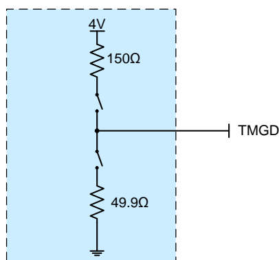
Figure 19. Output Equivalent Circuit for TMGD Pin
