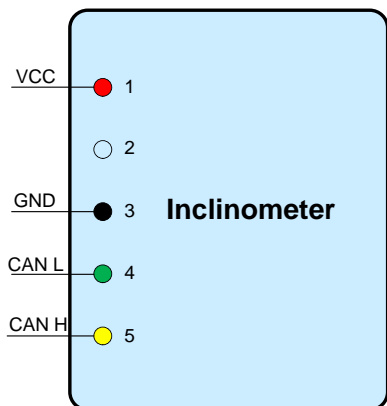
Figure 2. Pin Names
