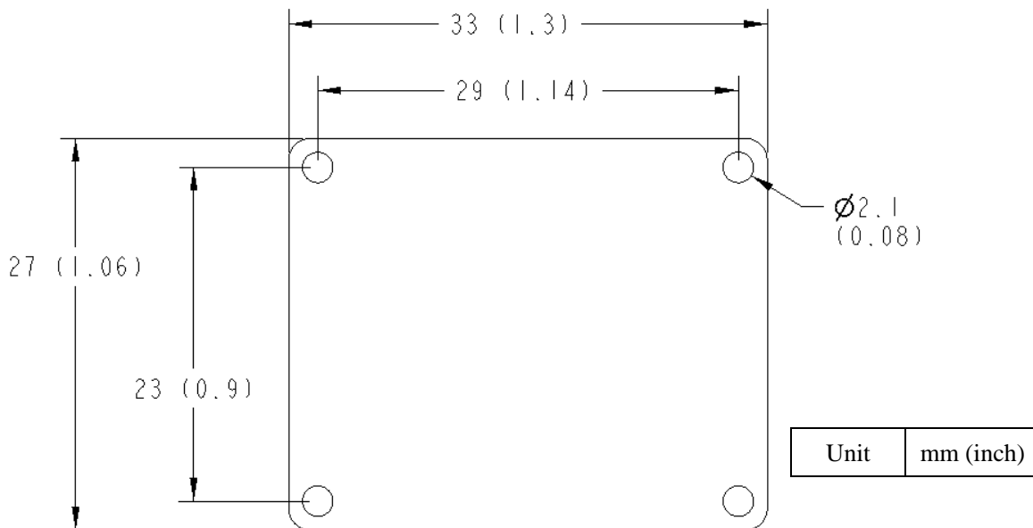
Figure 6. PCB Dimensions
