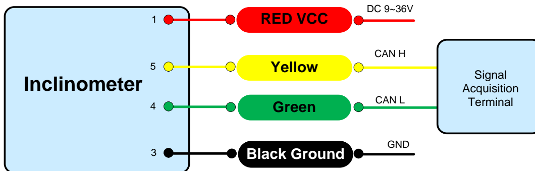
Figure 3. CAN BUS Wiring Diagram
