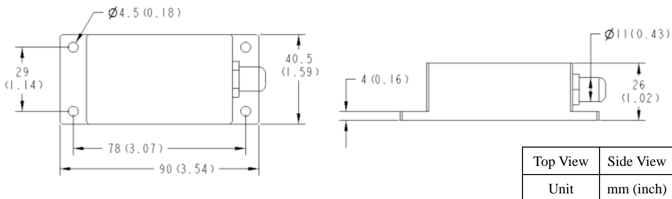
Figure 6. Outline Dimensions
