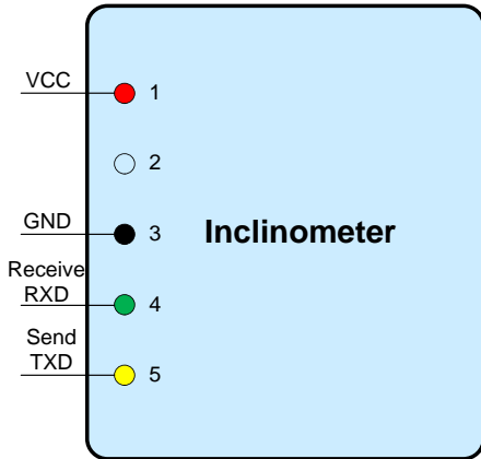
Figure 2. Pin Names
