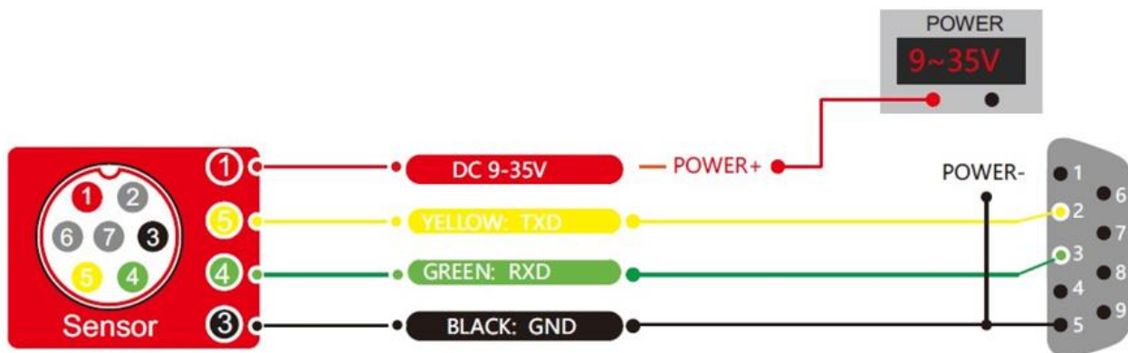
Figure 4. RS 232 Wiring Diagram
